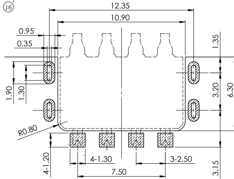
RECOMMENDED PCB LAYOUT TOLERANCE (.XX ± 0.05)
