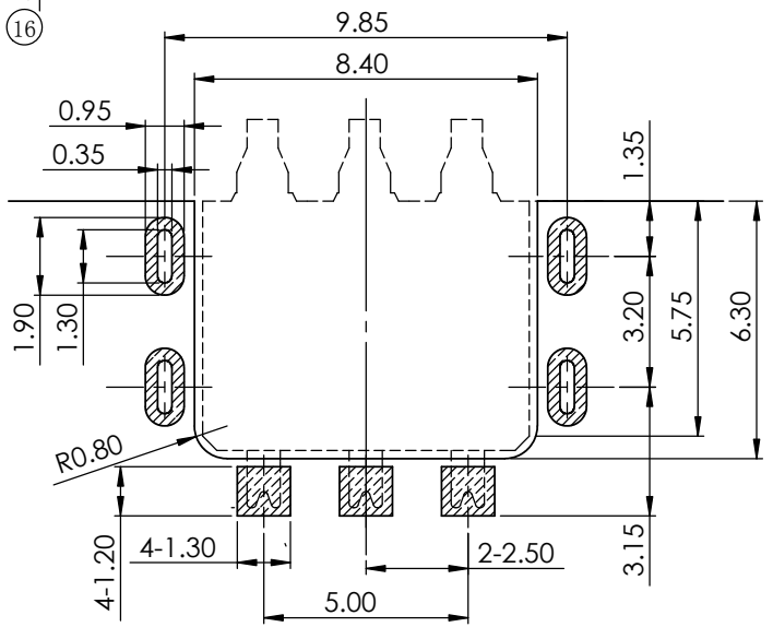
RECOMMENDED PCB LAOUT TOLERANCE (.XX ± 0.05)
